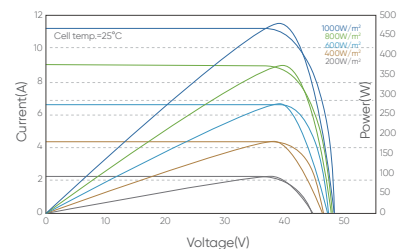
I-V/P-V Curve at Different Temperature (420W)
