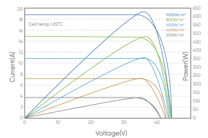
I-V/P-V Curve at Different Temperature (615W)
