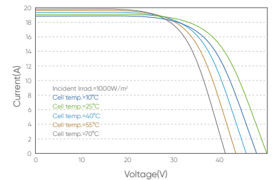
I-V Curve at Different Temperature (670W)
